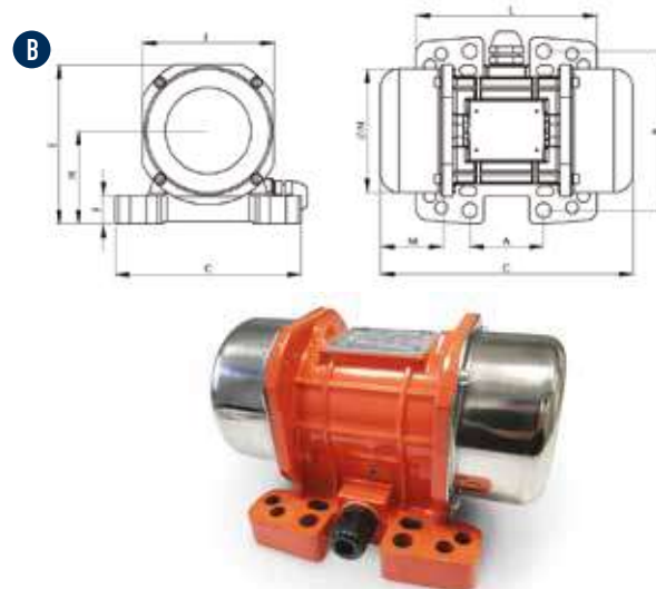
DIMENSIONAL SPECIFICATIONS
