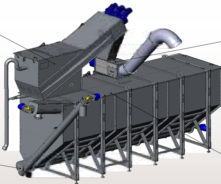
Jagged multi-screw with SINT® screen
